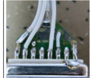
From left to right: Pin 8: Batterie plus Pin 7: Speaker + Pin 6: Mikrofon R Pin 5: Ext. NF Pin 4: Speaker minus (not GND) Pin 3: Mikrofon L Pin 2: TX Remote
